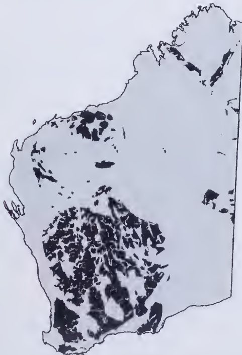
Figure 1. Distribution of granitoid landforms in Western Australia. Redrawn from the hydrogeological Map of Western Australia, Geological Survey of Western Australia (1989).
